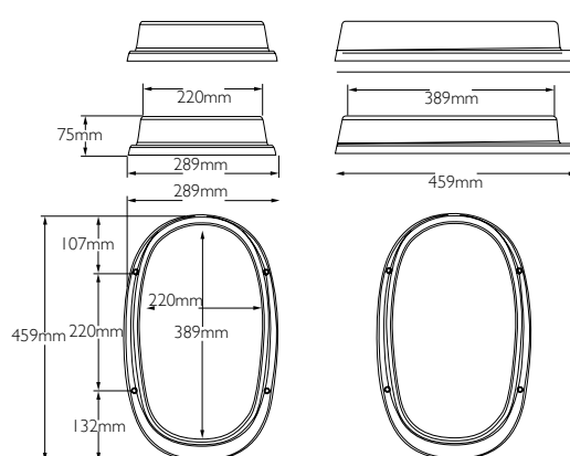
TP50/75/100BW back to wall design
