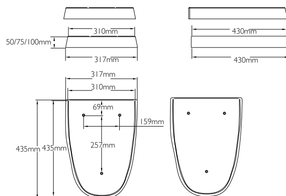
TP50/75/100BW back to wall design
