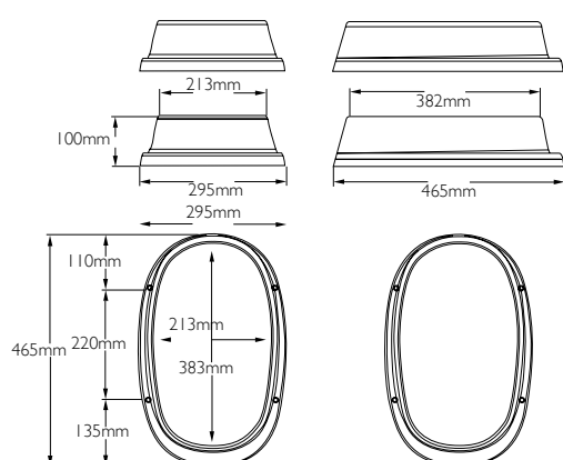
TP100 100 mm height
