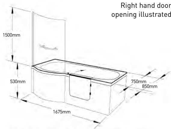
Available with left or right handed entry
