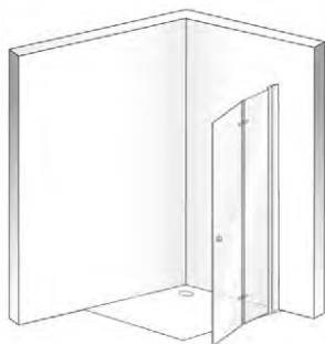
L5 (Right handed illustrated)
